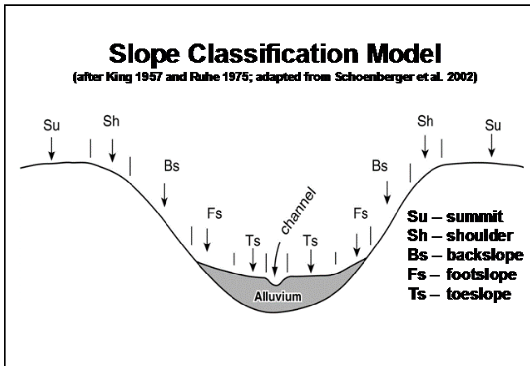
Figure 8. Idealized valley cross section showing Ruhe's slope elements (after Schoenberger et al. 2002).
