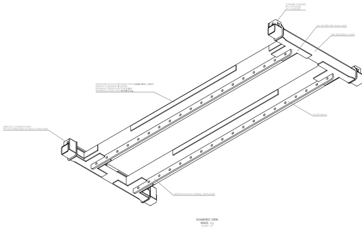
Image 05: Conceptual drawing outlines the first iteration of a purpose-built spreader frame.
