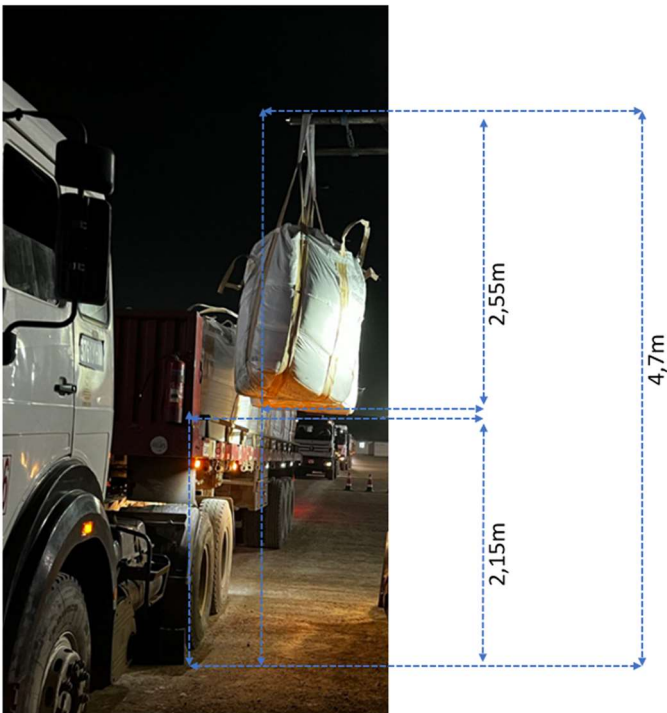
Image 02: Current process of lifting copper concentrate bags and approximate height of lifting.
